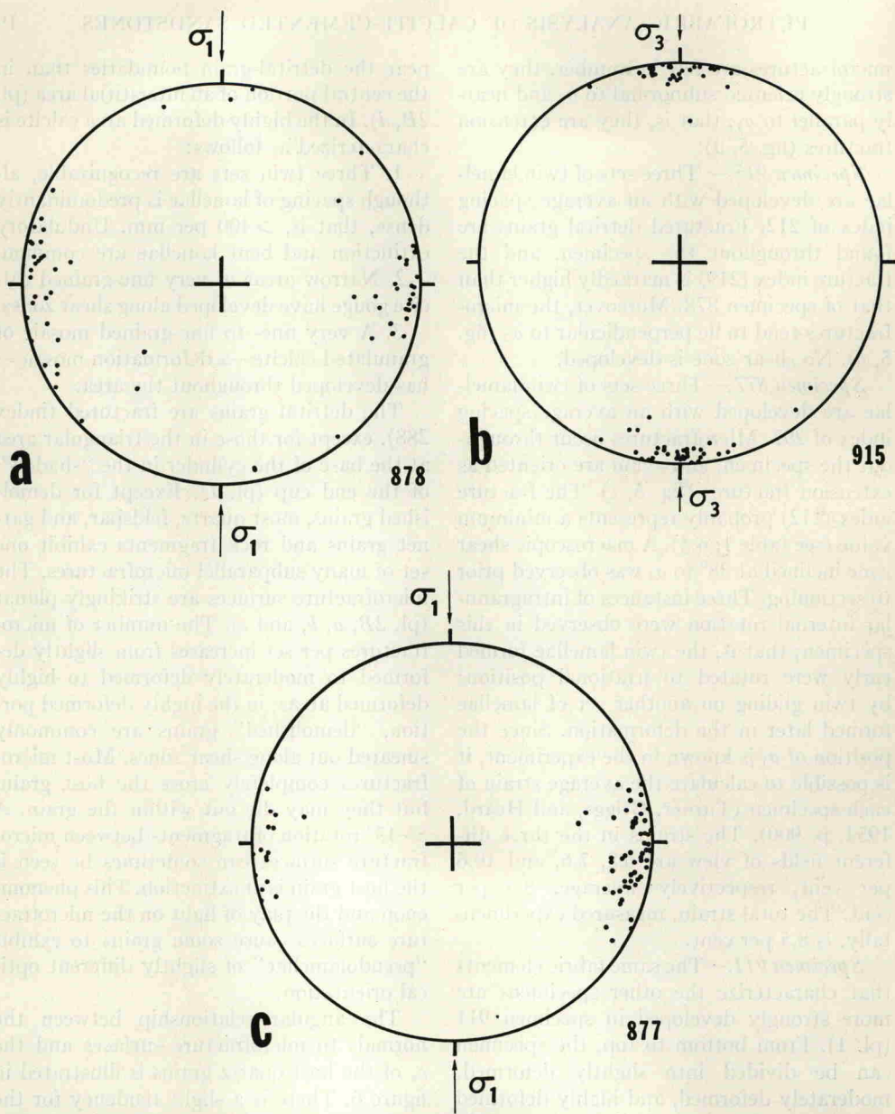
FIG. 5.—Diagrams illustrating orientation of microfractures with respect to load axis for specimens 878, 915, and 877. Plane of each diagram is parallel to long axis of deformed cylinder. a , specimen 878, normals to 63 sets of microfractures in fifty detrital grains. b , specimen 915, normals to 64 sets of microfractures in fifty detrital grains. c , specimen 877, normals to 69 sets of microfractures in fifty detrital grains.
